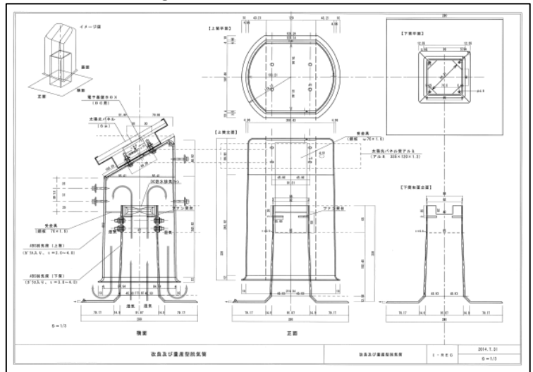
[Product Drawing]
